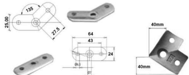
HH1001K-H Straight Saddle 304/316 HH1001-H45 45 Degree Saddle 304/316 HH1001K-Z 90 Degree Saddle 304/316
