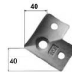
HH1001K-Z-50.8 90 Degree Angle Saddle 30/316
