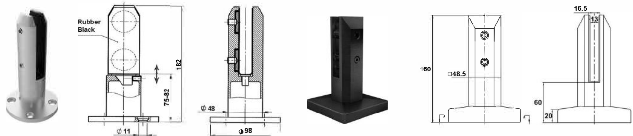
GLH1082 Round Spigot (Cover Available) 316G Satin To Suit 12-17.52mm Glass
