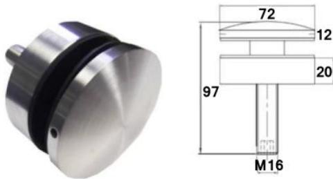
JK-1019 Solid Threaded Body – Convex Head M16 Removable Thread 304/316
