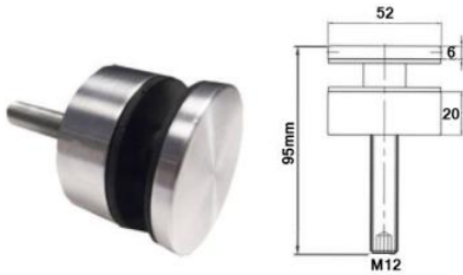
JK-1015 Solid Threaded Body – Flat Head M12 Removable Thread 304/316
