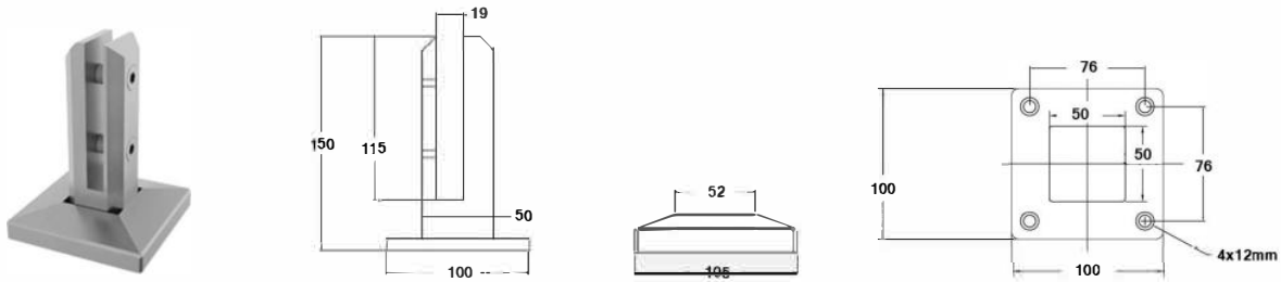
GLH1090 Square Spigot & Base (Rubbers for 10 and 12mm) 316G Mirror
