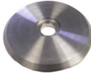
RON1006-50-14.5K 8.5mm Hole 14.5mm Recess 304/316
