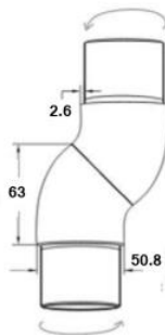
RV1007/50.8 45/135 Degree Set Angle Connector 316
