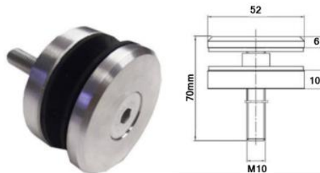
JK-1012 Solid Threaded Body – Screw Head M10 Removable Thread 304/316
