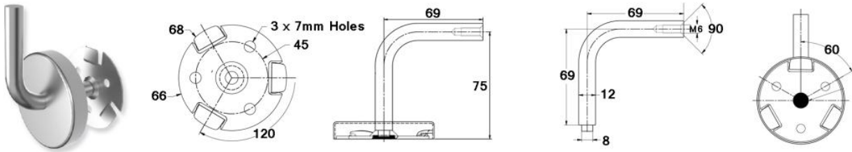
KT-Twist-Lock-75mm 75mm Off-Set Twist and Lock Handrail Bracket 304 and 316G - Satin
