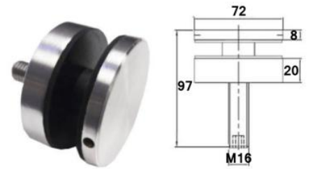
JK-1016 Solid Threaded Body – Flat Head M16 Removable Thread 304/316
