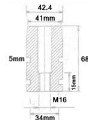
BDH1005-120x3-42.4 Smaller 68mm Spigot x 120mm Plate 304/316
