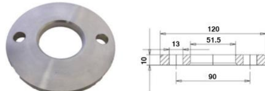
RON1010/50.8 Weldable Plate 304/316
