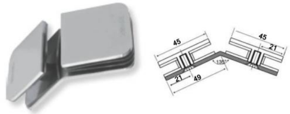
KT-SGC-202-S4 / KT-SGC-202-(04)M Glass to Glass Connector 135D 304G Satin / 304G Mirror
