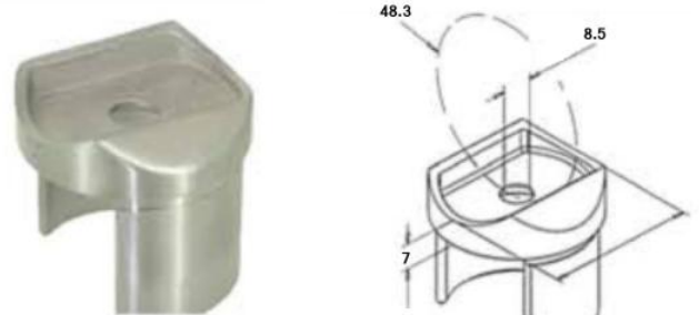
1503.483.304/316 Slotted Adaptor 304/316
