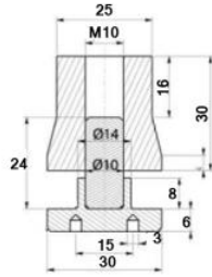
GLH1013K-30 Solid Threaded Body - Pig Nose M10 Removable Thread 316
