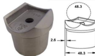
48-RA1006 Adaptor 304/316
