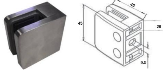
KLH10F-45/45-Zintec St/St Effect - 10mm Glass Zamack Glass Clamp (No Pin)
